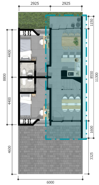
1 st Floor
